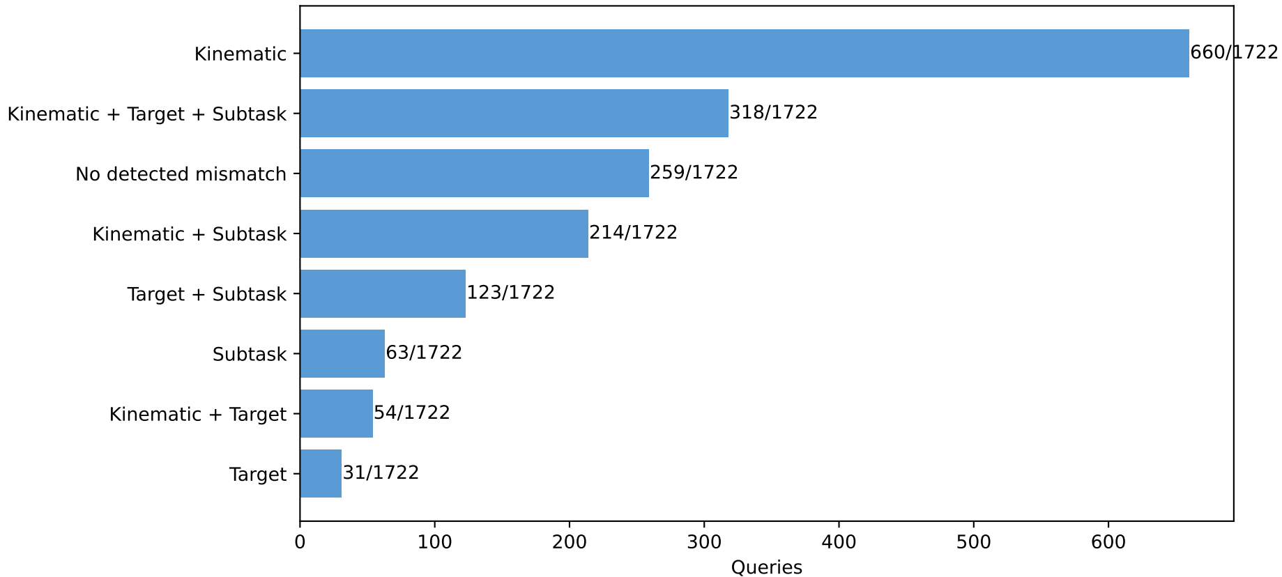
Mismatch co-occurrence Kinematic \times Target \times Subtask; 90 tasks \times 1 trial
