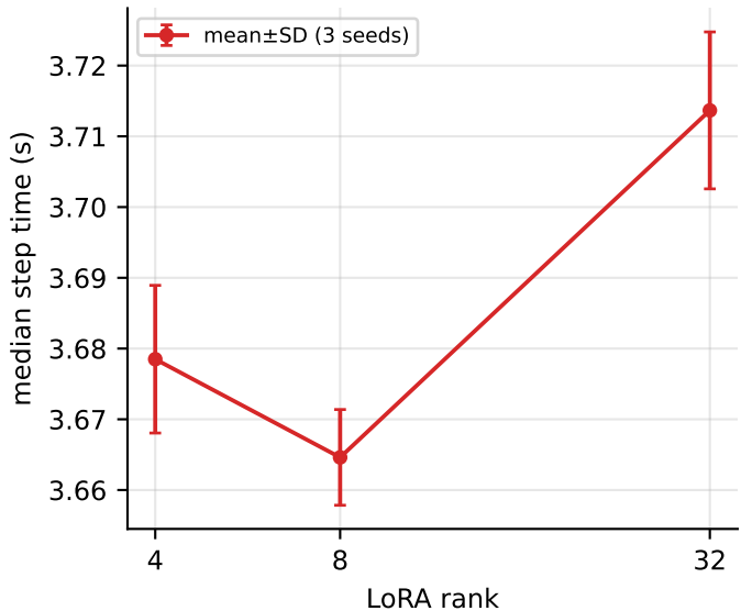
Step time vs LoRA rank (4B-4bit, ctx512)
