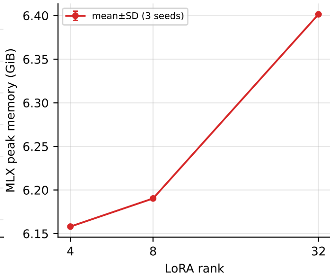
Peak memory vs LoRA rank (4B-4bit, ctx512)
