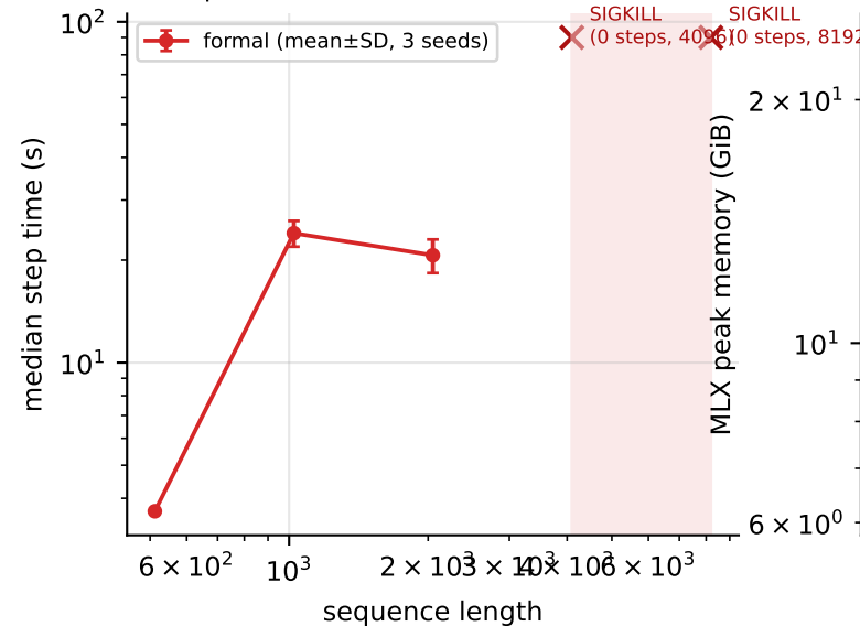
Step time vs context (4B-4bit QLoRA, b1)
