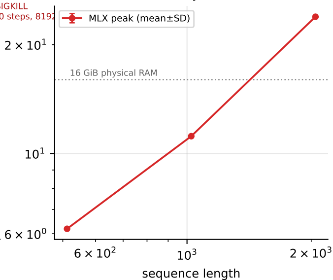
Peak memory vs context
