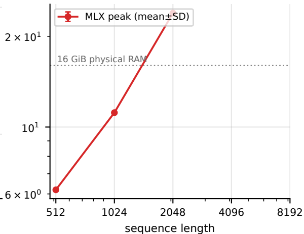
Peak memory vs context
