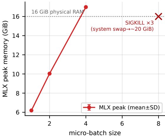
Peak memory vs batch (batch boundary \in [4,8) )
