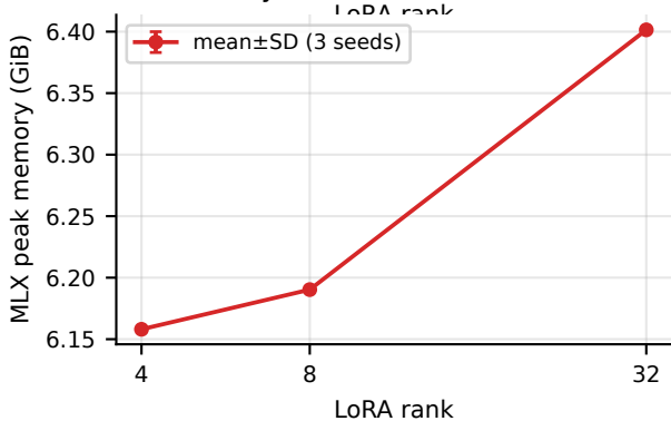
Peak memory vs LoRA rank (4B-4bit, ctx512)
