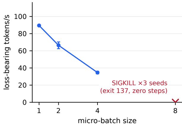
Throughput vs batch (4B-4bit, ctx512)
