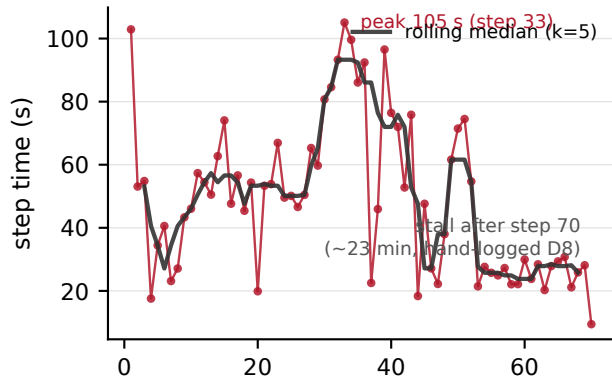
(a) 14B 4-bit timeout run: 70/100 steps
