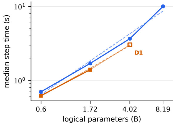
Step time vs scale
