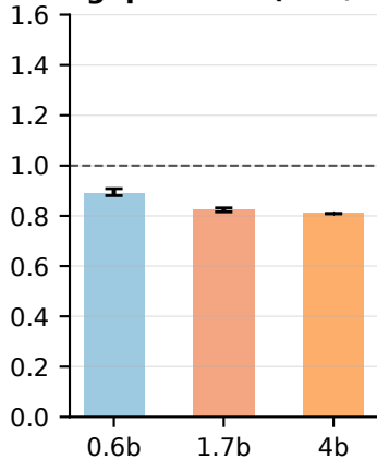
throughput ratio (4bit/BF16)
