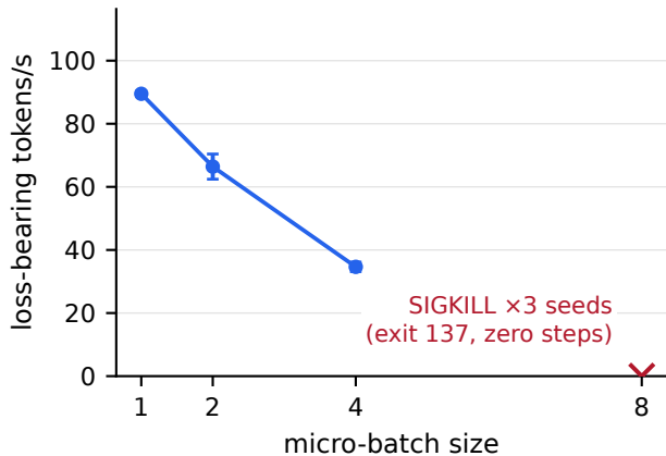
Throughput vs batch (4B-4bit, ctx512)
