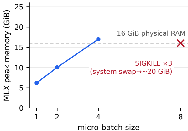
Peak memory vs batch (batch boundary ∈ [4,8))
