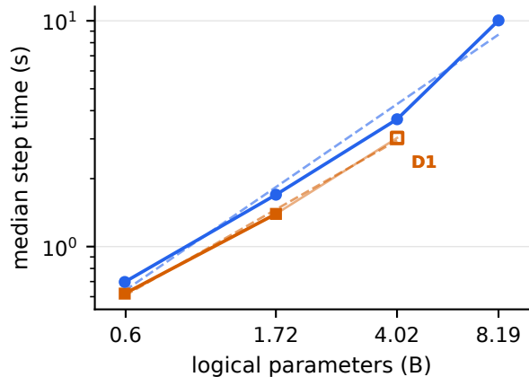
Step time vs scale
