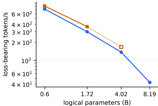
Throughput vs scale
