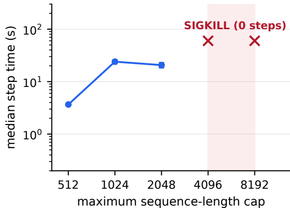
Step time vs cap (4B-4bit QLoRA, b1)
