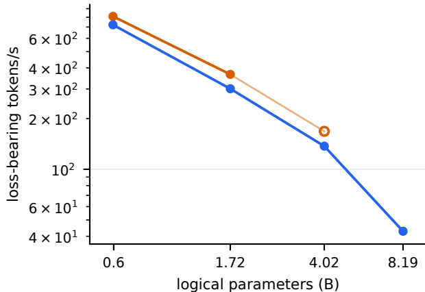
Throughput vs scale
