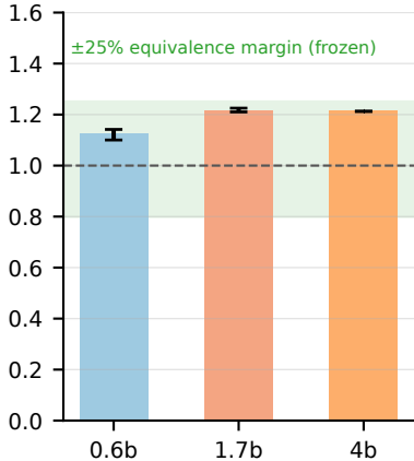
step-time ratio (4bit/BF16)
