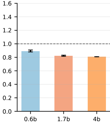
throughput ratio (4bit/BF16)
