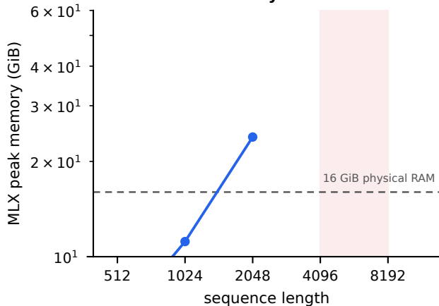
Peak memory vs context
