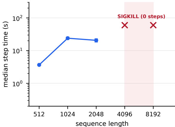
Step time vs context (4B-4bit QLoRA, b1)
