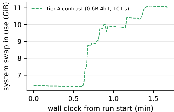
(c) batch-8 runs: swap ramp to SIGKILL (0 steps)
