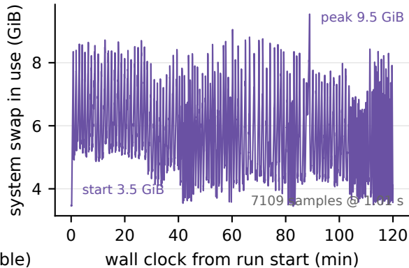
(b) same run: 1 Hz sampled swap (saw-tooth)
