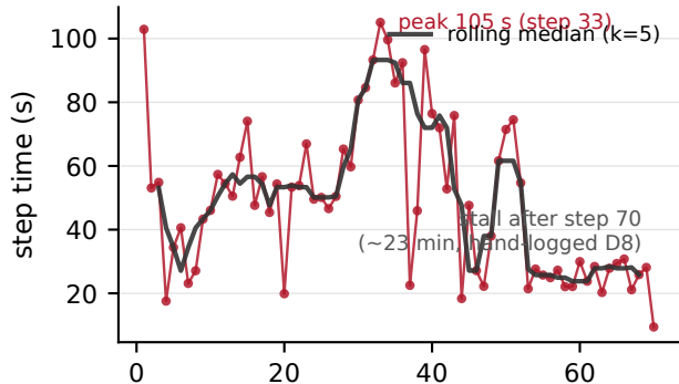
(a) 14B 4-bit timeout run: 70/100 steps
