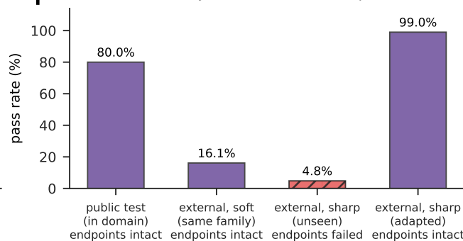
f Pass rate by model-domain competence
