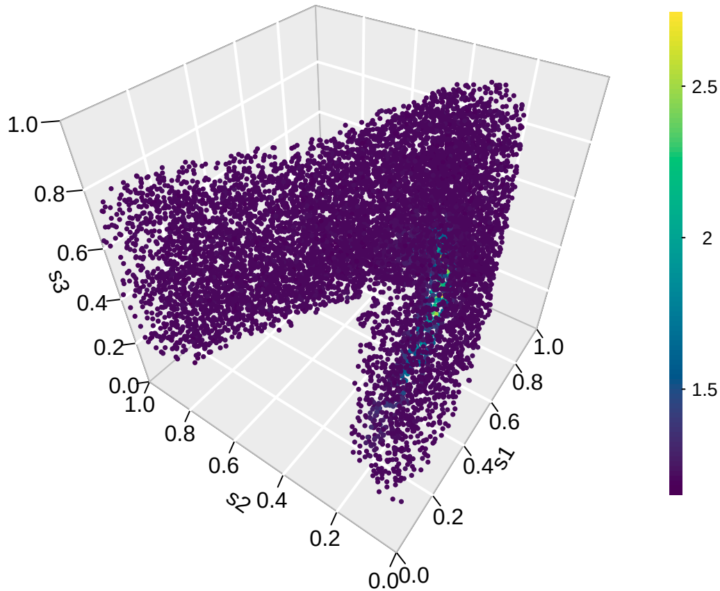
gene61 (focal)
