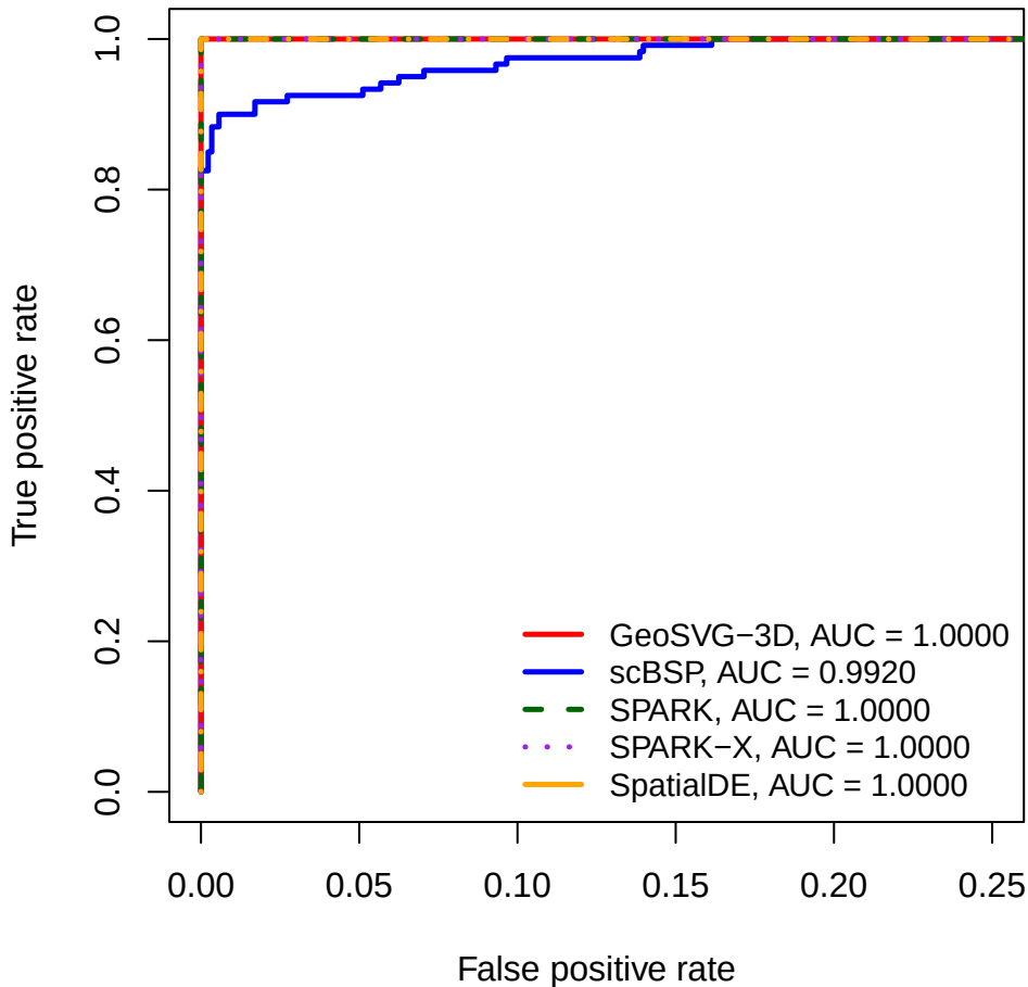
(a) ROC curve
