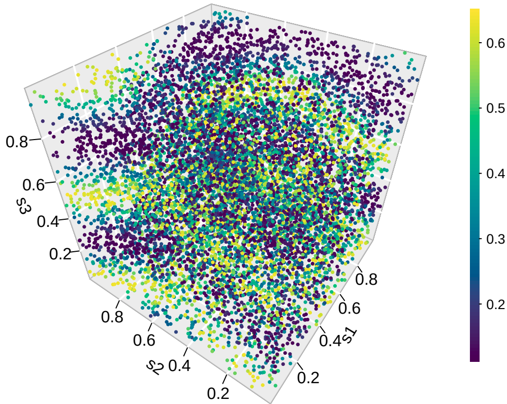
gene101 (complex)
