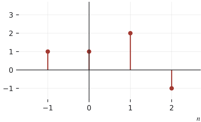
impulse response h[n]
