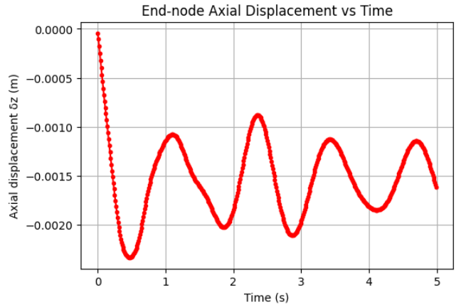
Fig. 3. End-node axial displacement \delta_z(t) over time
