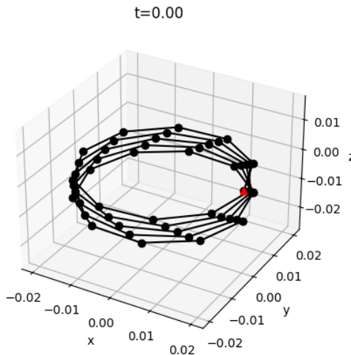
Fig. 1. Initial undeformed helical spring configuration at t = 0
