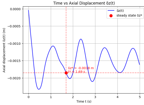
Fig. 4. End-node axial displacement \delta_z(t) over time with steady-state
