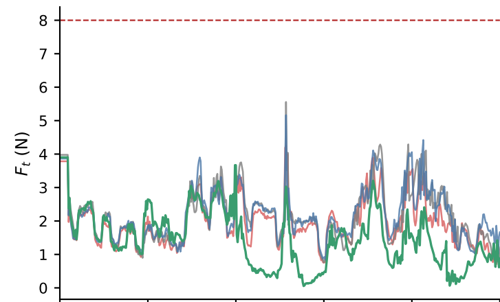
Path 7 (coupling gel)
