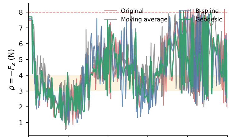
Path 7 (coupling gel)
