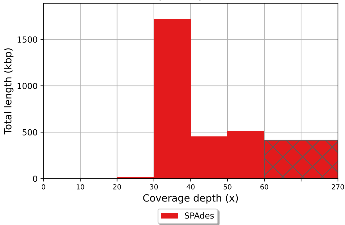
SPAdes coverage histogram (bin size: 10x)
