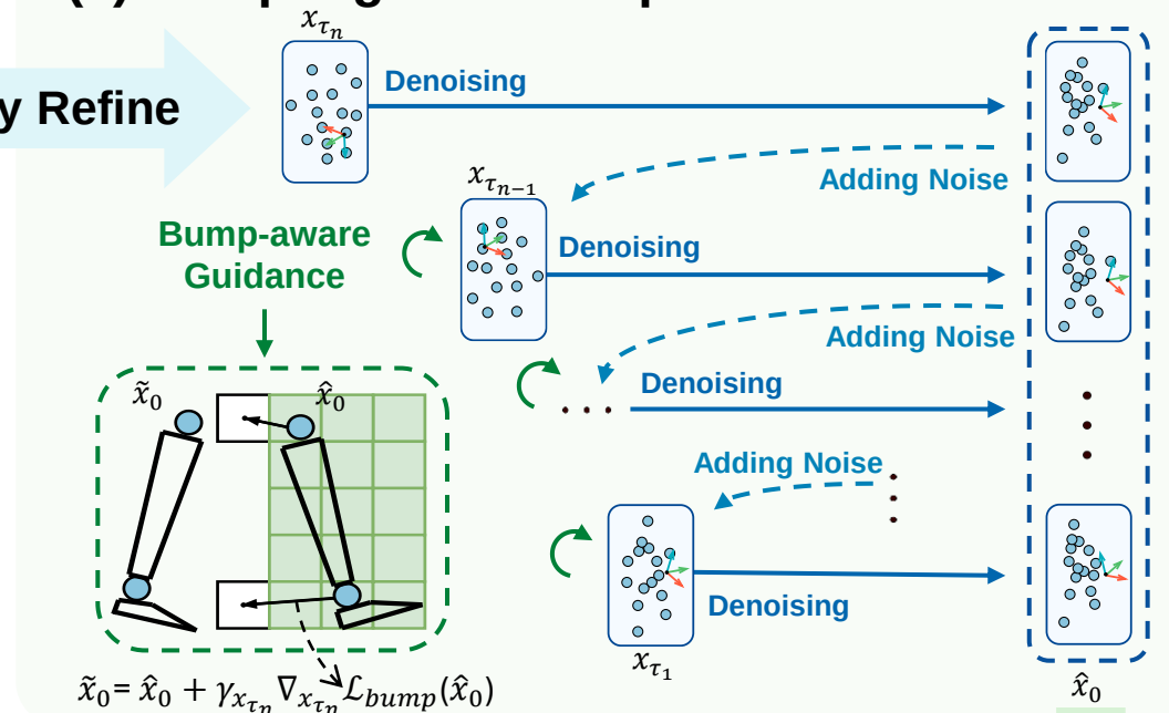
(c) Sampling with Bump-aware Guidance
