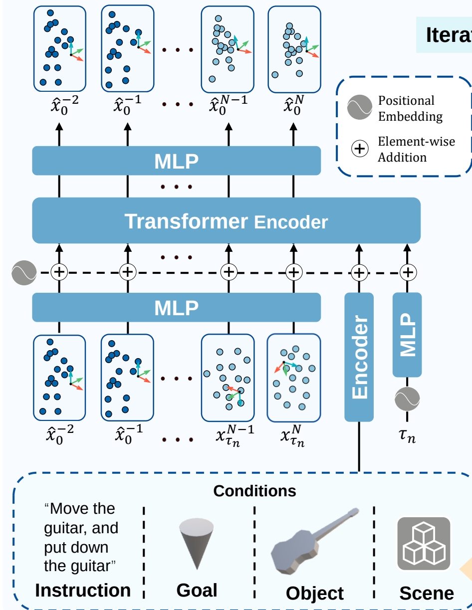
(a) Auto-regressive Motion Model
