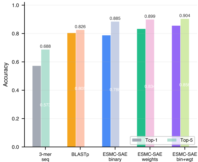
EC3 prediction (161 classes, 974 test)
