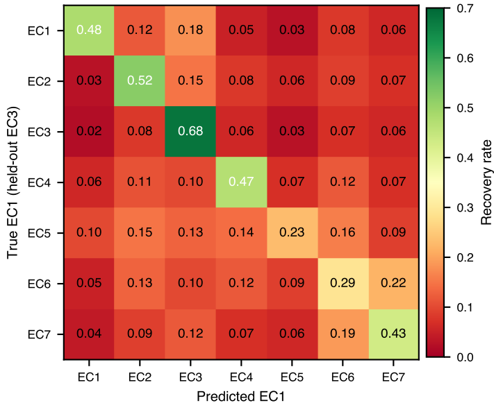
EC1 recovery — ESMC-SAE binary
