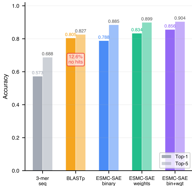
Full method comparison
