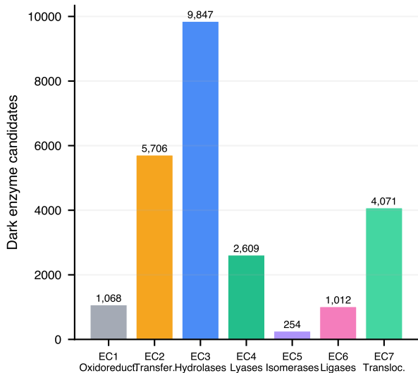
Dark enzyme-like clusters (total: 24,567)
