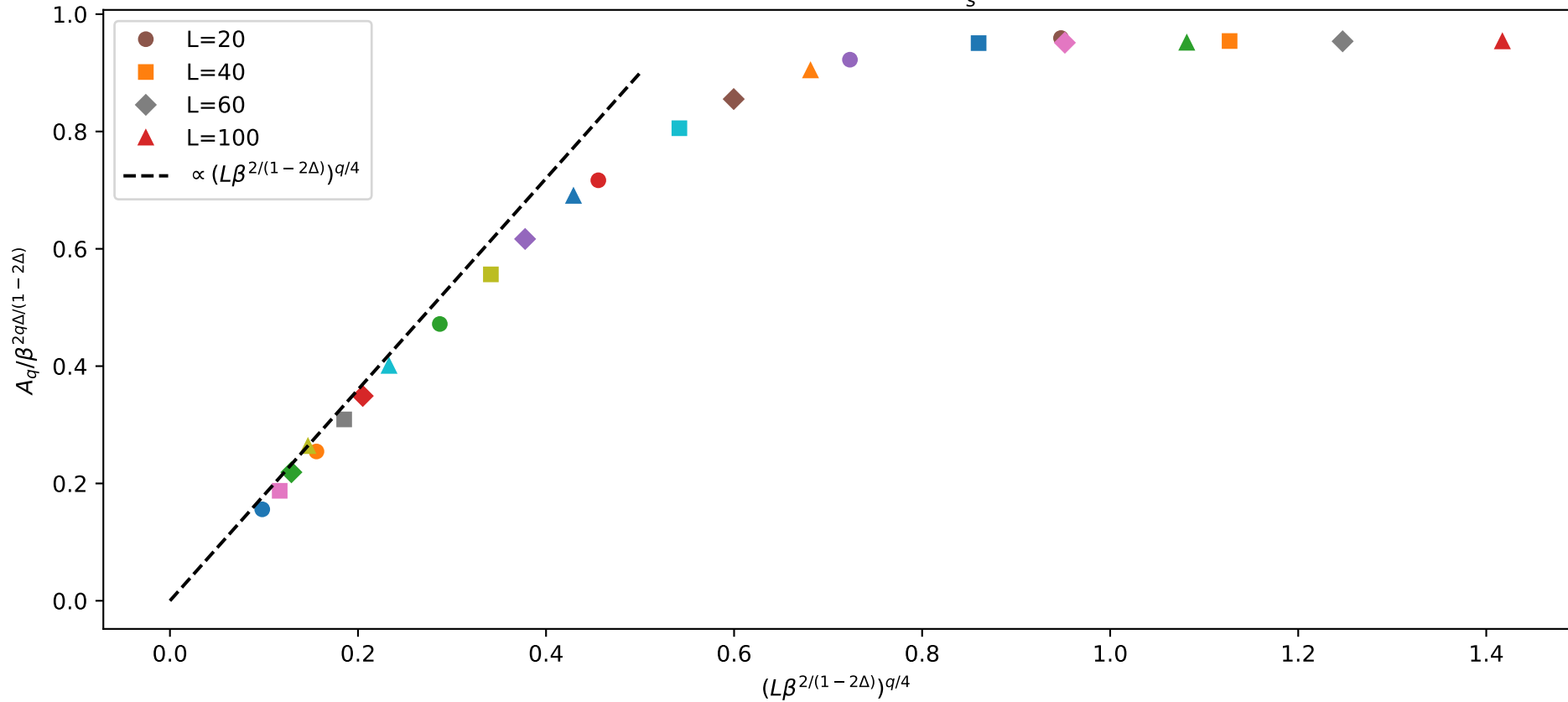
Majority Vote Classifier: Finite-size scaling of A_q : = \sum_s p(s) |\langle Z \rangle_s|^q with q = 1 for \beta \leq 0.3
