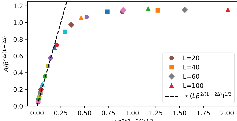
Finite-size scaling for \beta \leq 0.3
