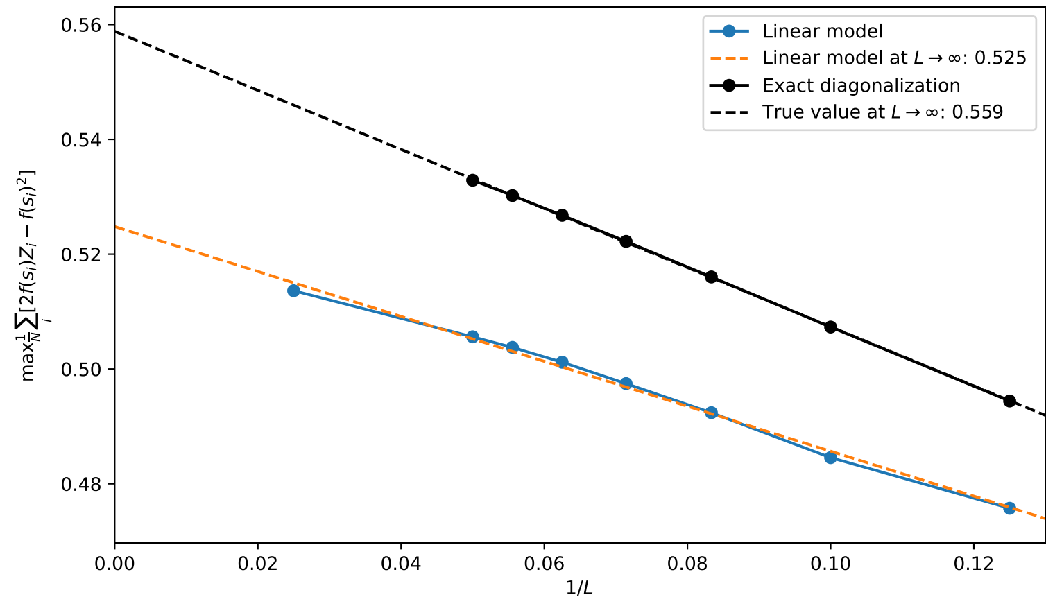
Relative error at L \rightarrow \infty : -6.1 %
