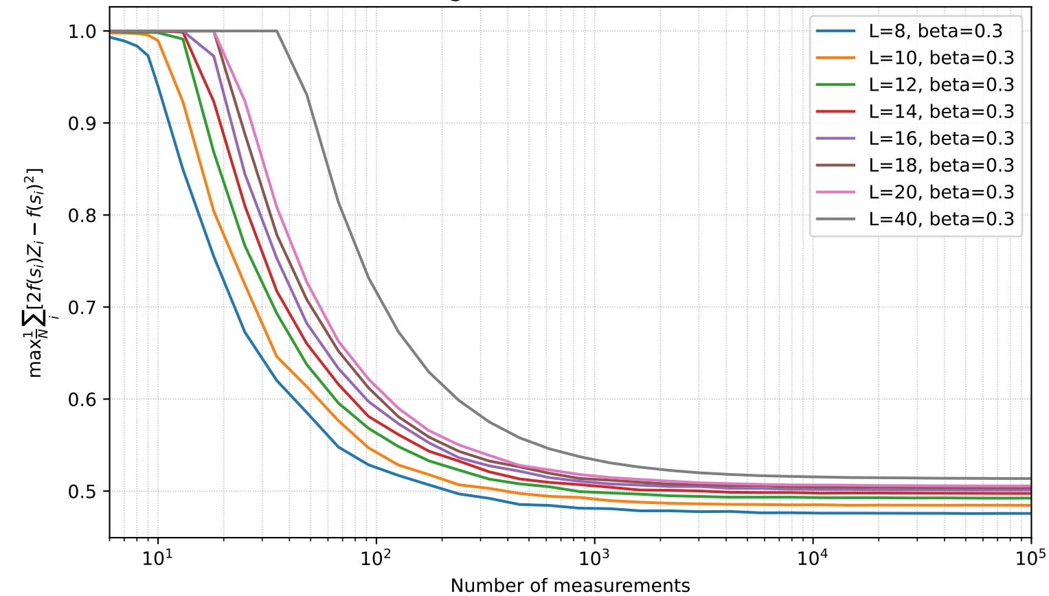
Critical Ising, Z measurements, beta=0.3
