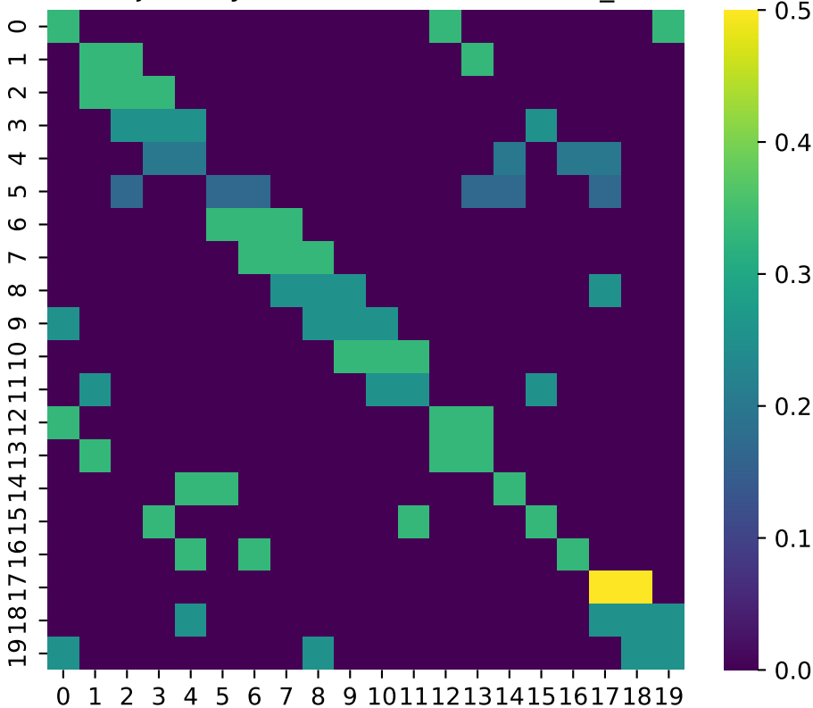
Adjacency (Transition) Matrix - mat 9
