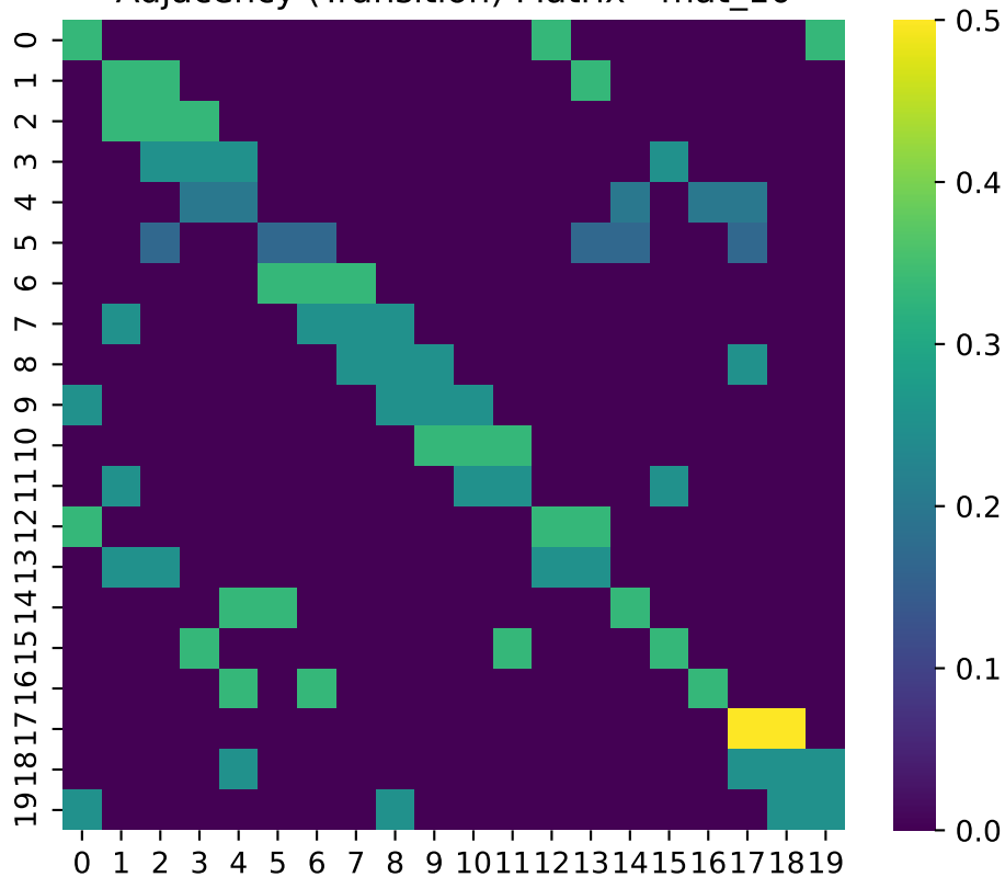
Adjacency (Transition) Matrix - mat_10
