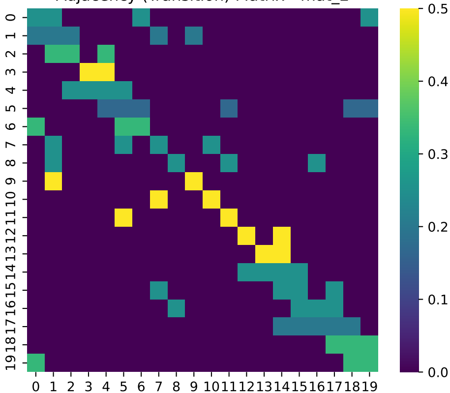
Adjacency (Transition) Matrix - mat_2
