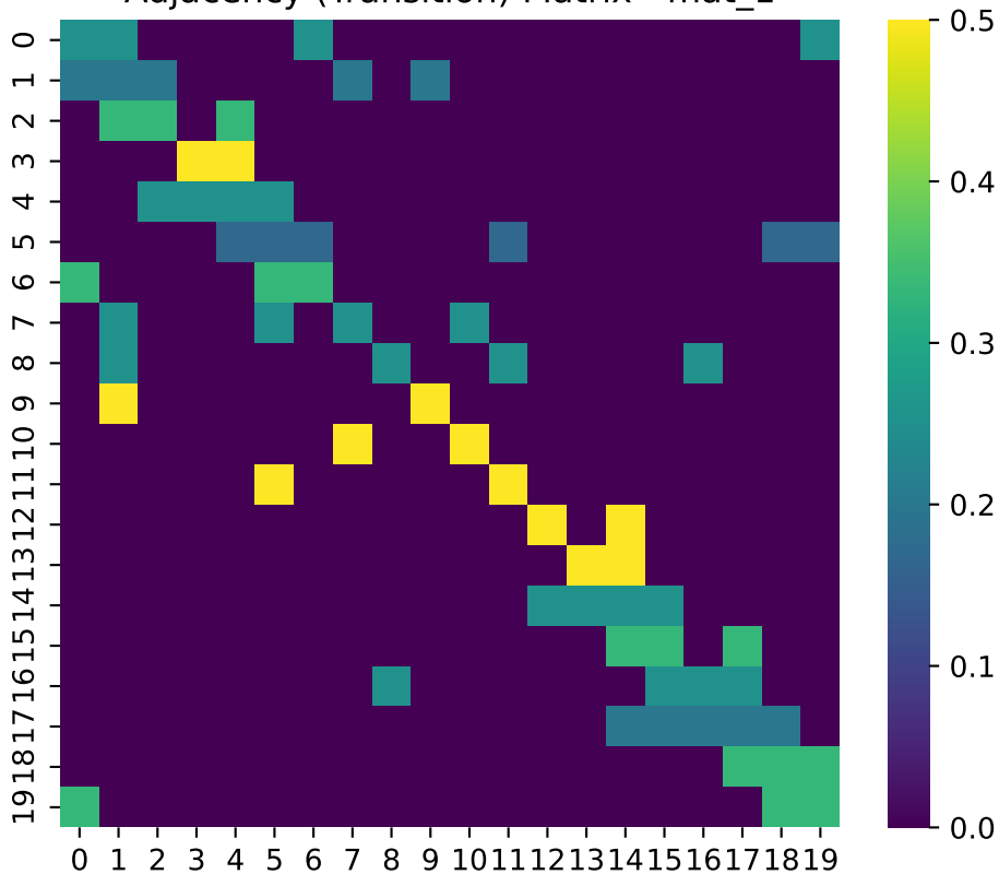
Adjacency (Transition) Matrix - mat_1
