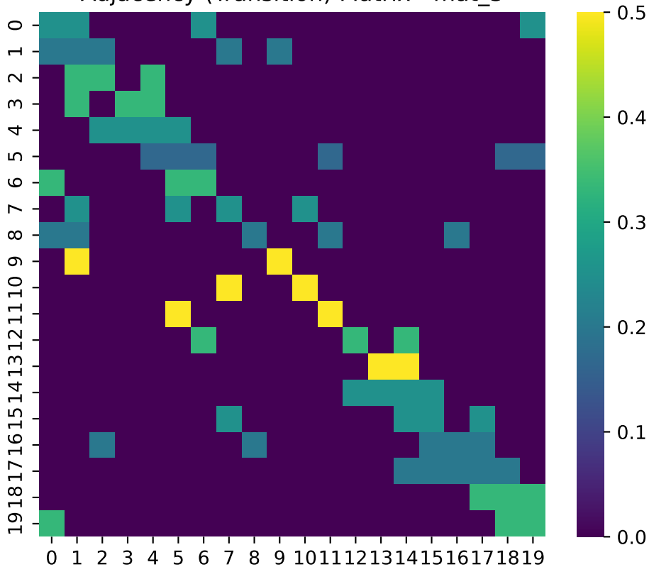
Adjacency (Transition) Matrix - mat_3
