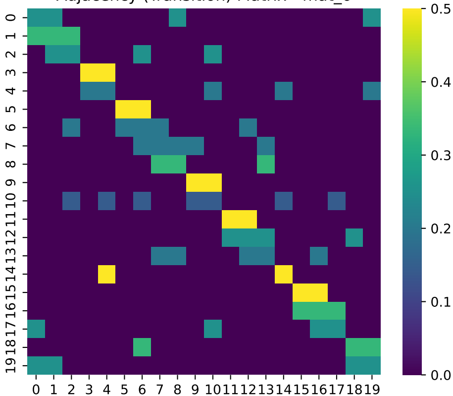
Adjacency (Transition) Matrix - mat_6
