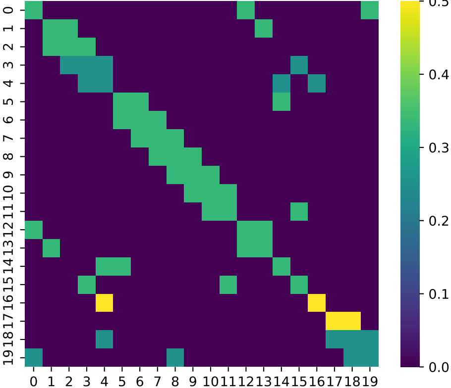
Adjacency (Transition) Matrix - mat 8
