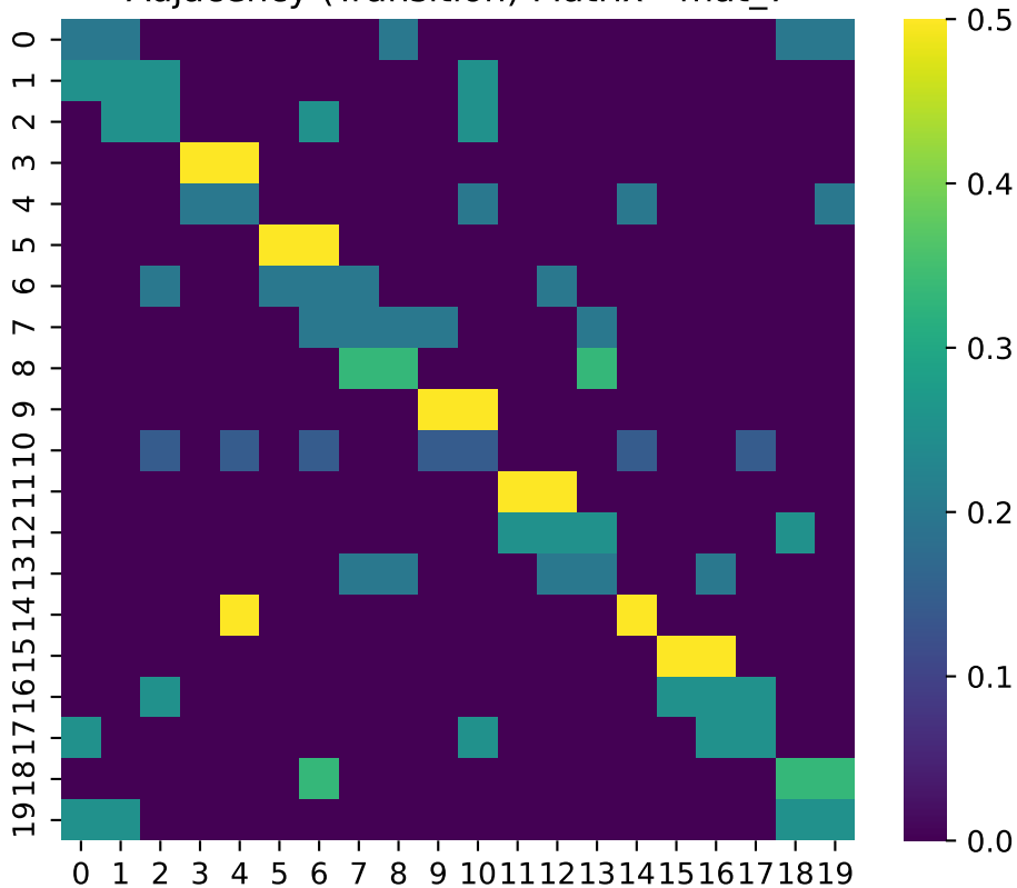
Adjacency (Transition) Matrix - mat_7
