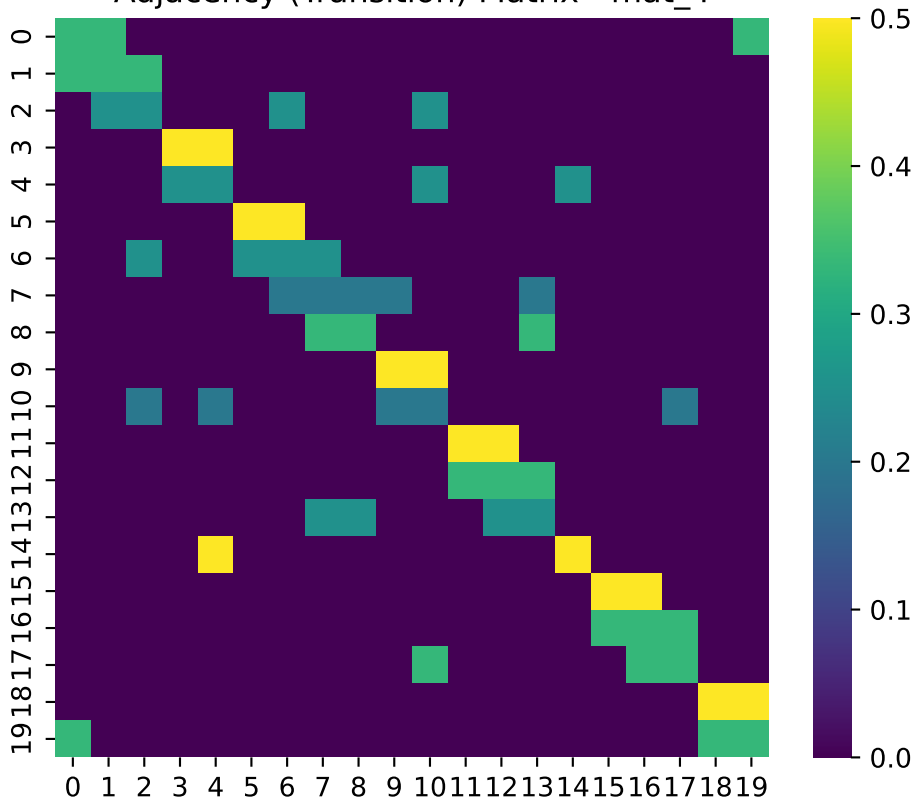
Adjacency (Transition) Matrix - mat_4
