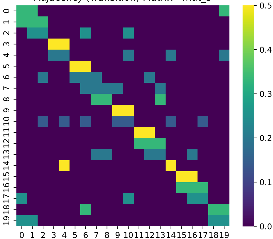
Adjacency (Transition) Matrix - mat_5
