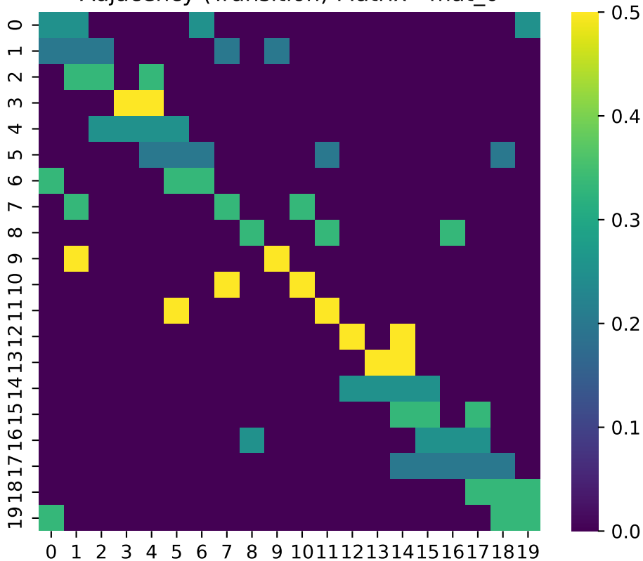
Adjacency (Transition) Matrix - mat_0
