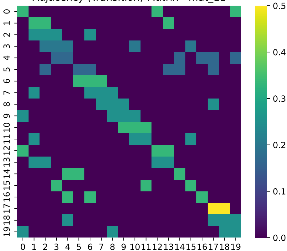
Adjacency (Transition) Matrix - mat_11
