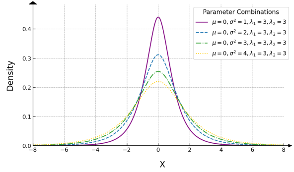
(b) \mu = 0, \sigma^2 = 1, 2, 3, 4, \lambda_1 = 3 and \lambda_2 = 3
