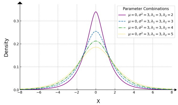
(d) \mu = 0, \sigma^2 = 3, \lambda_1 = 3 and \lambda_2 = 2, 3, 4, 5
