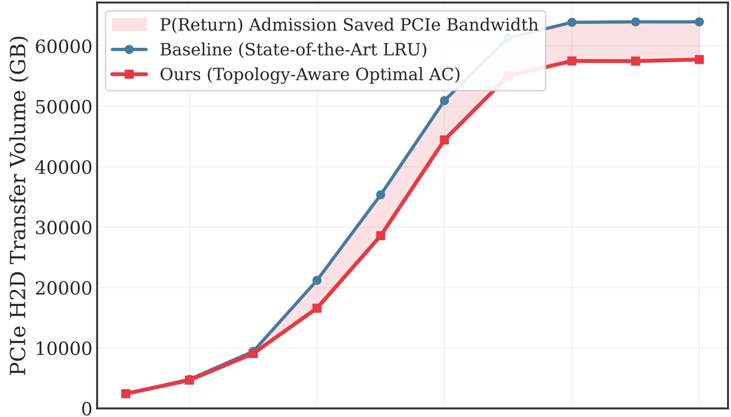
DeepSeek (Spectral Gap \delta = 0.925 )
