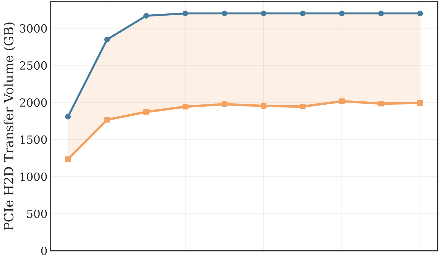
Mixtral (Spectral Gap \delta = 0.858 )
