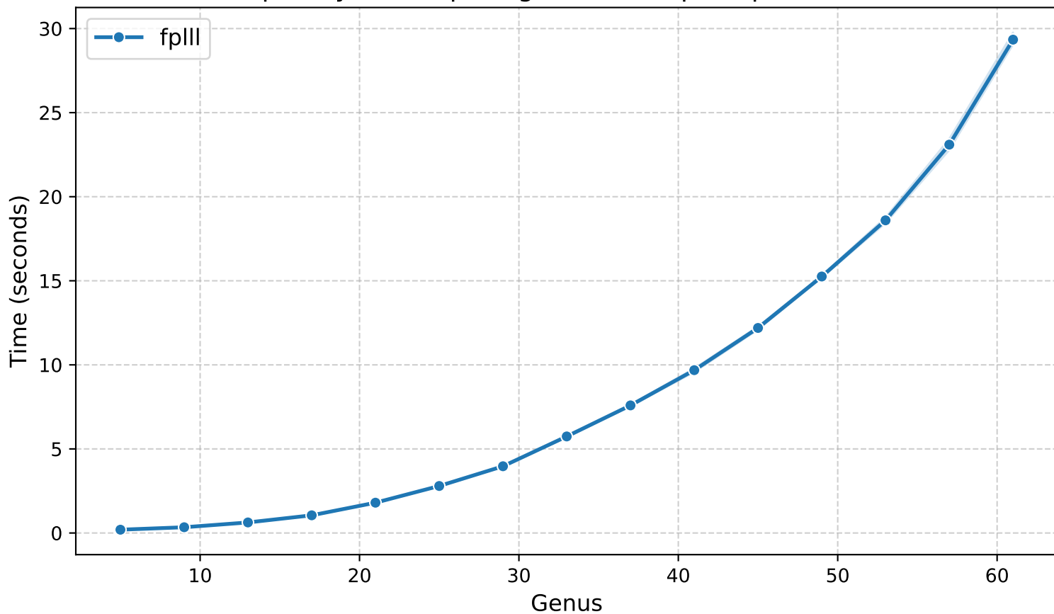
Time complexity of computing the full tropical polarization matrix
