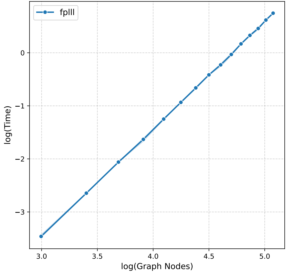
Time complexity of computing the full tropical polarization m
