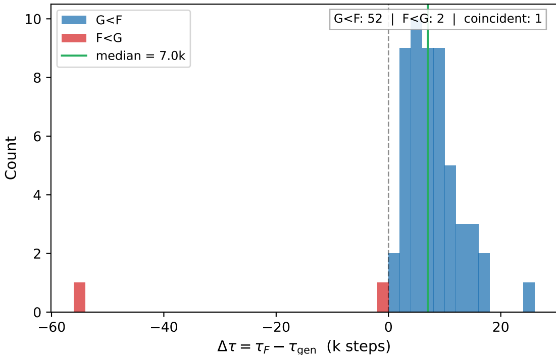
\Delta\tau distribution — addition p = 53 (Stage 2+3, n = 55 Grokking runs)
