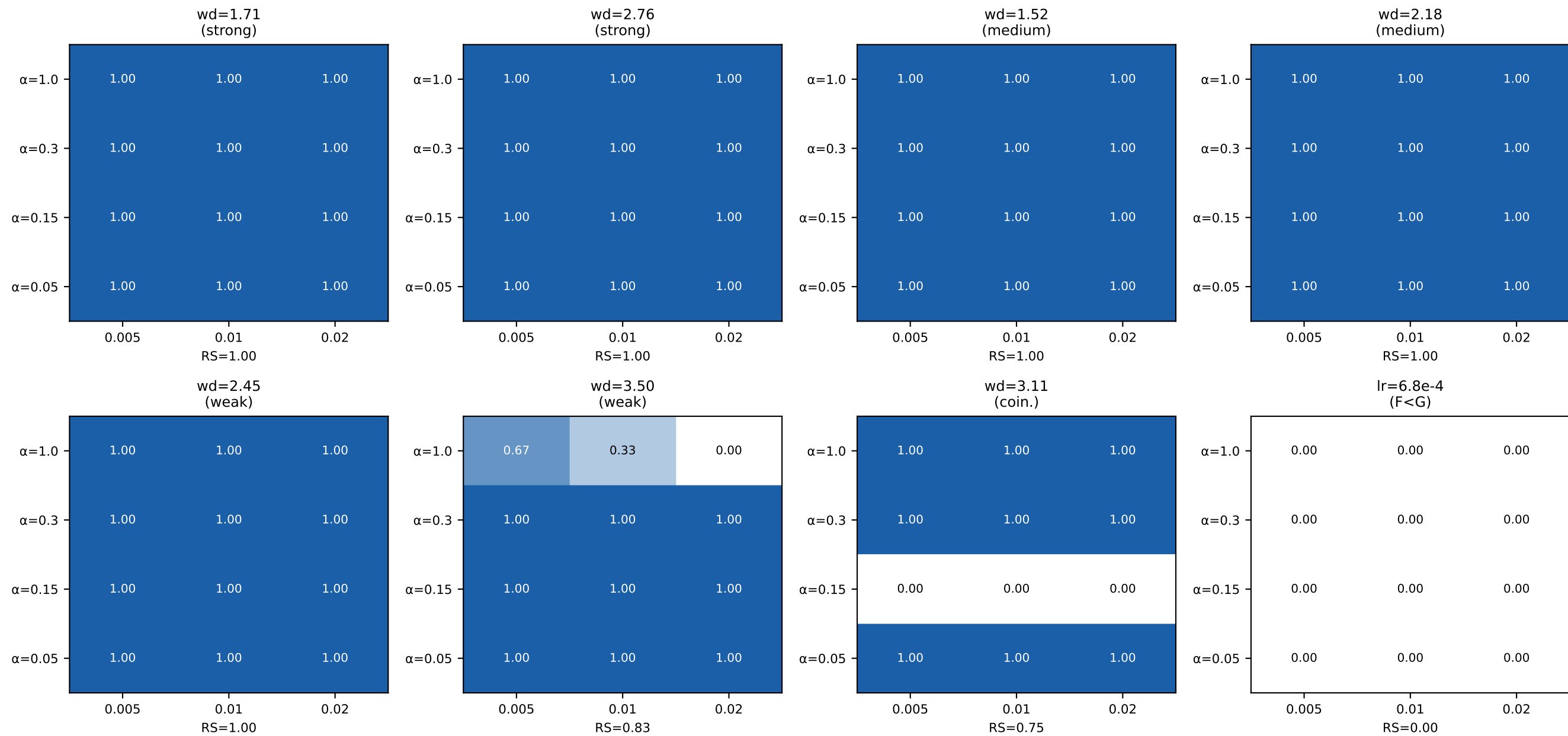
Per-cell P(G&lt;F) across detector configurations (marginalized over null_interval)
