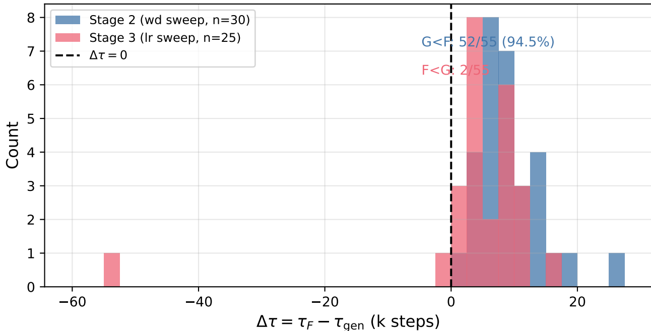
Distribution of \Delta\tau across 55 Grokking runs
