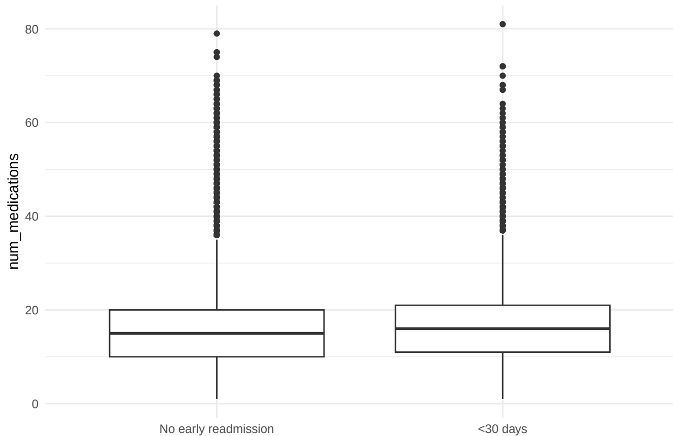
Distribution of num_medications by early readmission status
