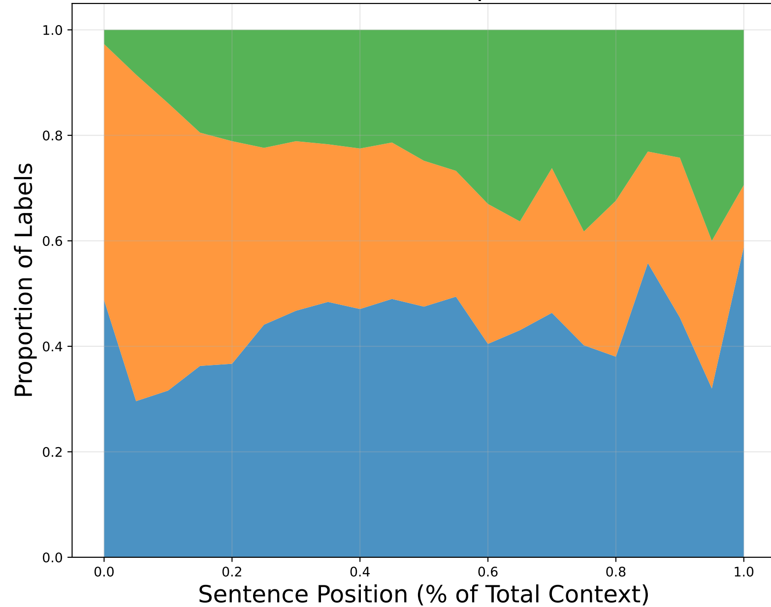
GPT-4o Self-Reported
