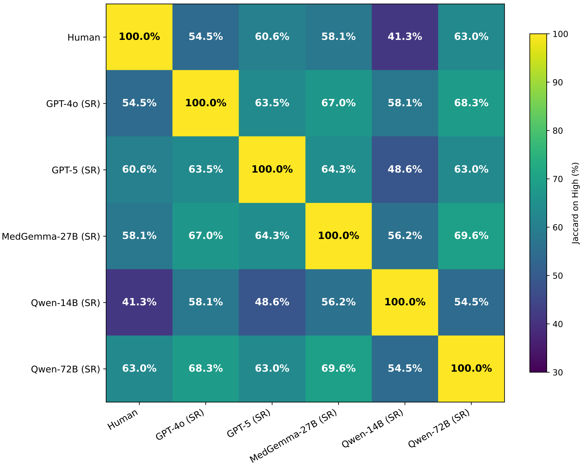
High-Relevance Concordance (Jaccard) SR = Self-Reported · n=933 QAs
