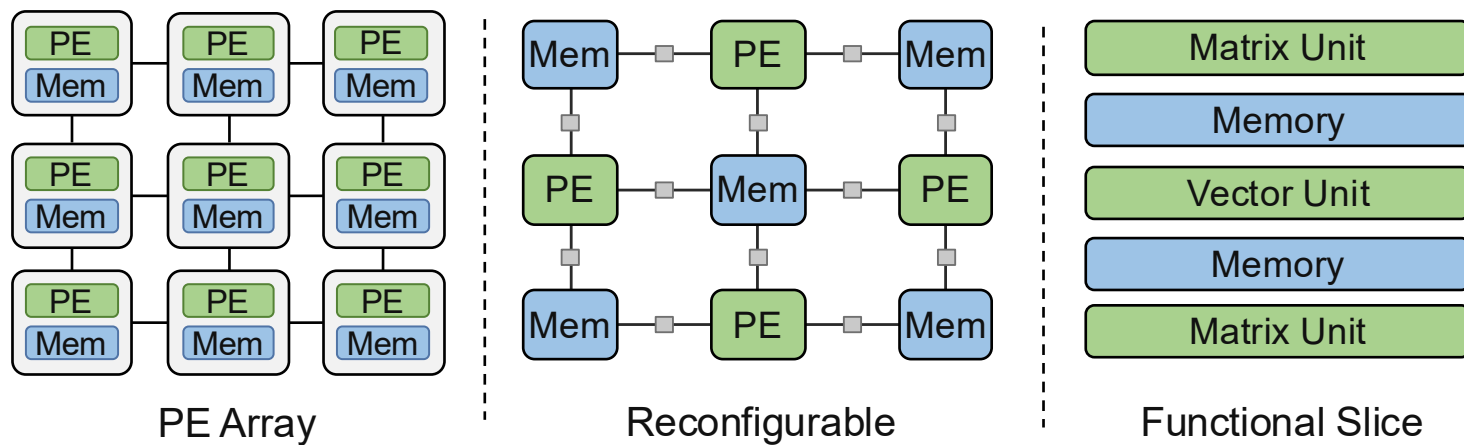
(c) Spatial Dataflow
