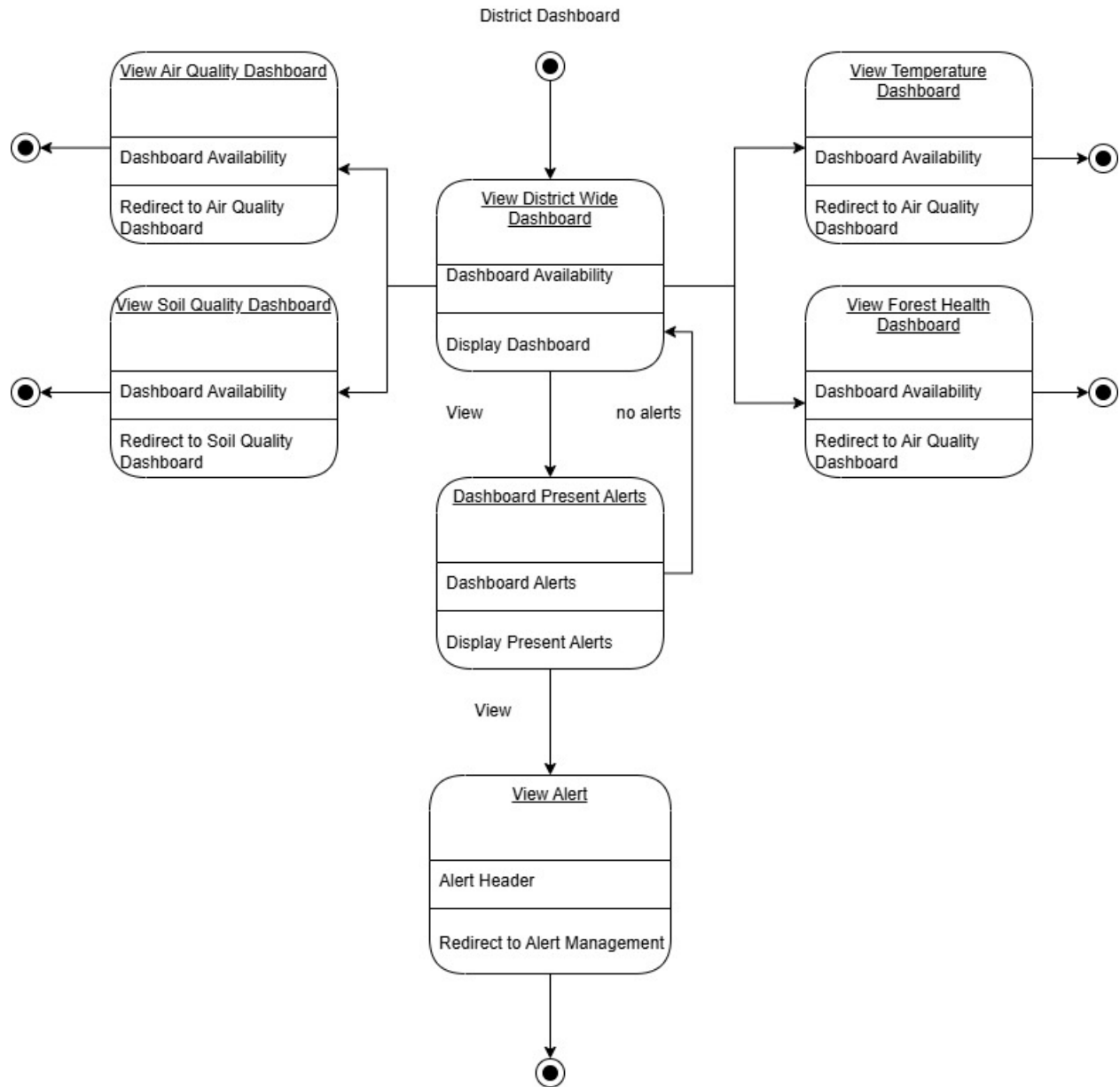
Figure 3: State diagram for District Dashboard Controller
