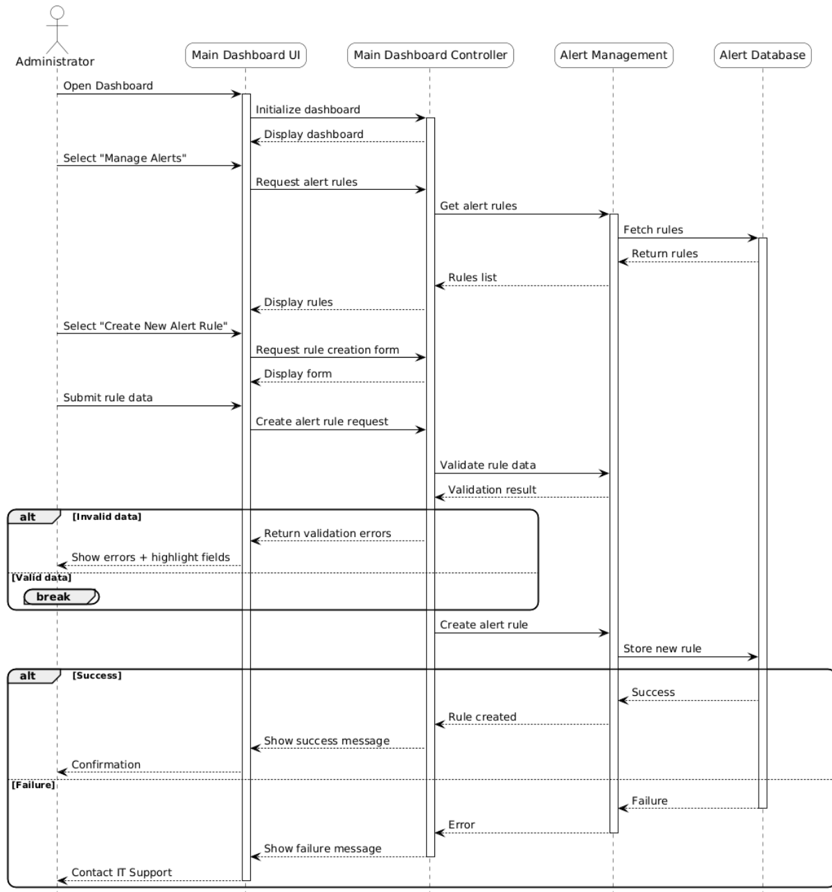
Figure 12: Sequence diagram for creating a new alert rule
