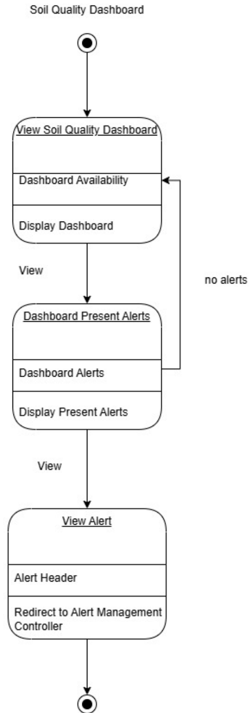
Figure 5: State diagram for Soil Quality Dashboard Controller
