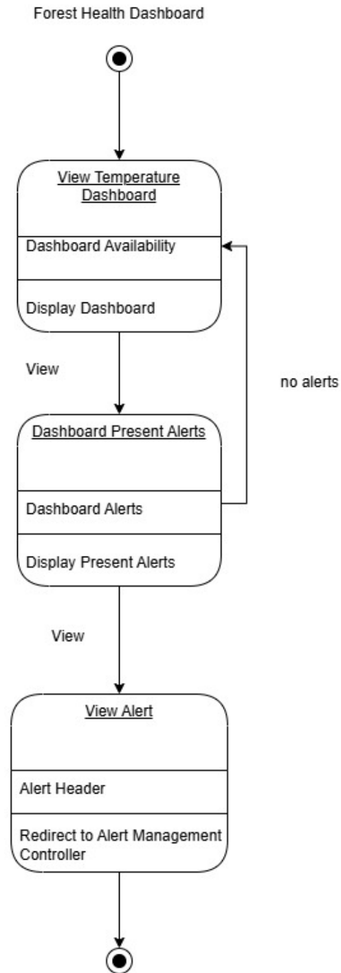
Figure 4: State diagram for Forest Health Dashboard Controller
