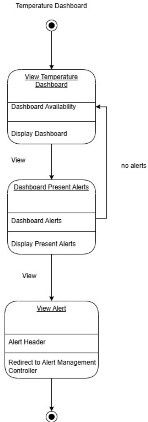
Figure 7: State diagram for Temperature Dashboard Controller
