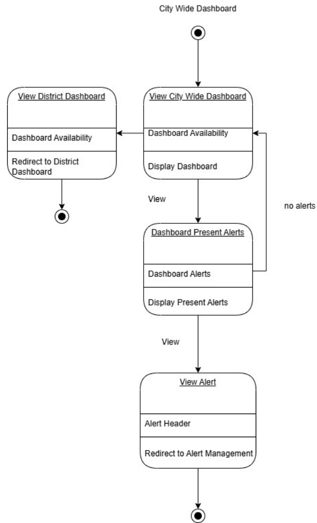
Figure 2: State diagram for City Dashboard Controller
