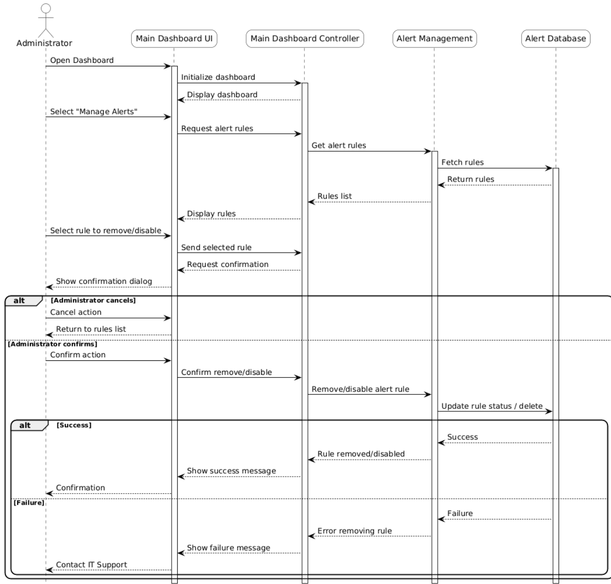
Figure 14: Sequence diagram for removing/disabling an existing alert rule
