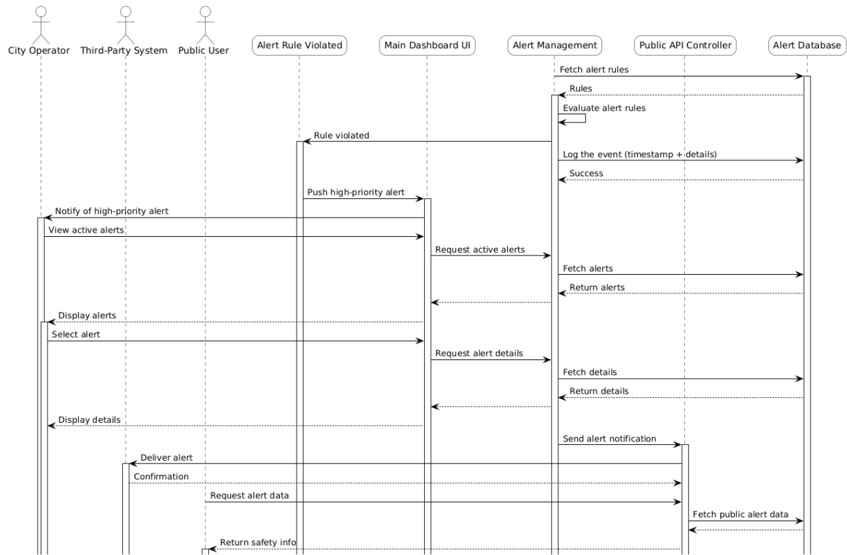
Figure 15: Sequence diagram for detecting a rule violation
