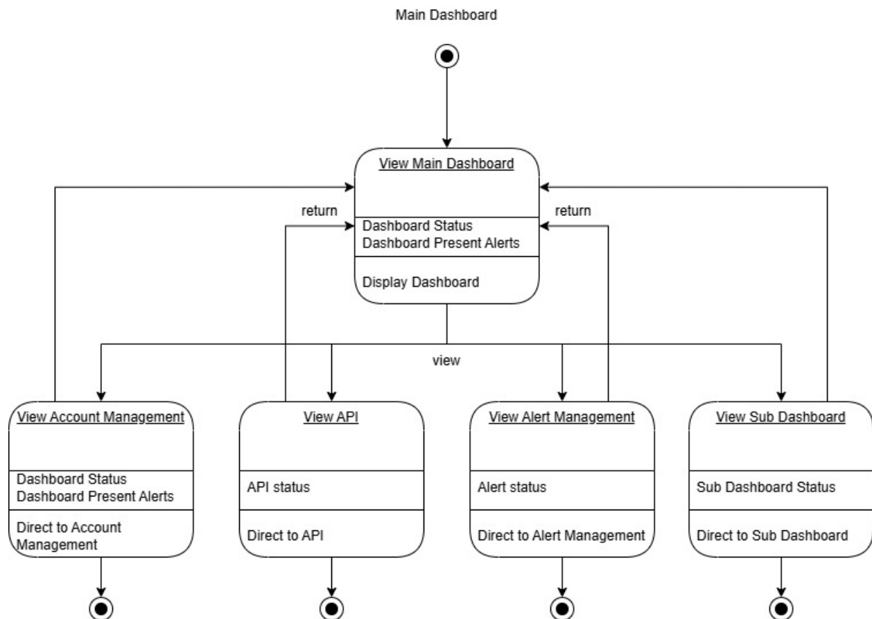
Figure 1: State diagram for Main Dashboard Controller
