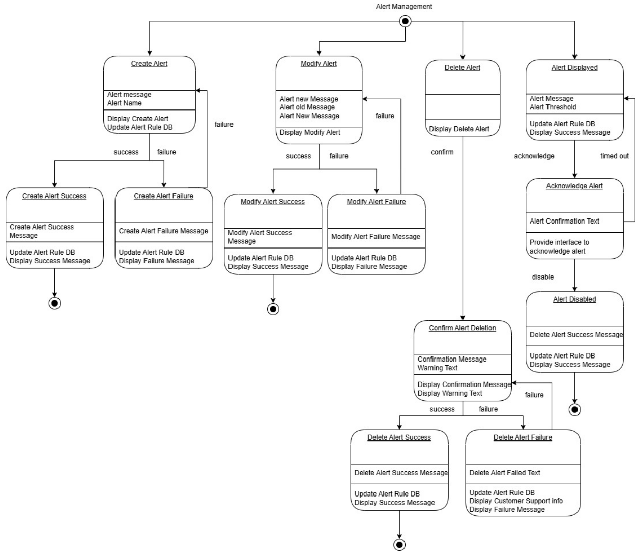
Figure 8: State diagram for Alert Management Controller
