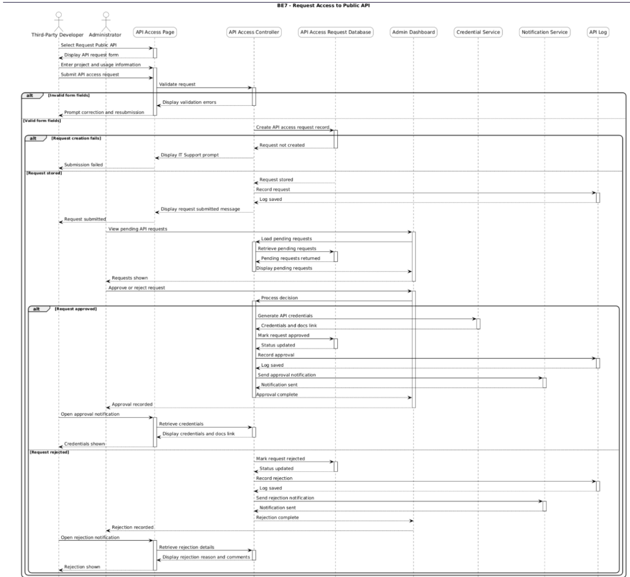
Figure 18: Request access to public API
