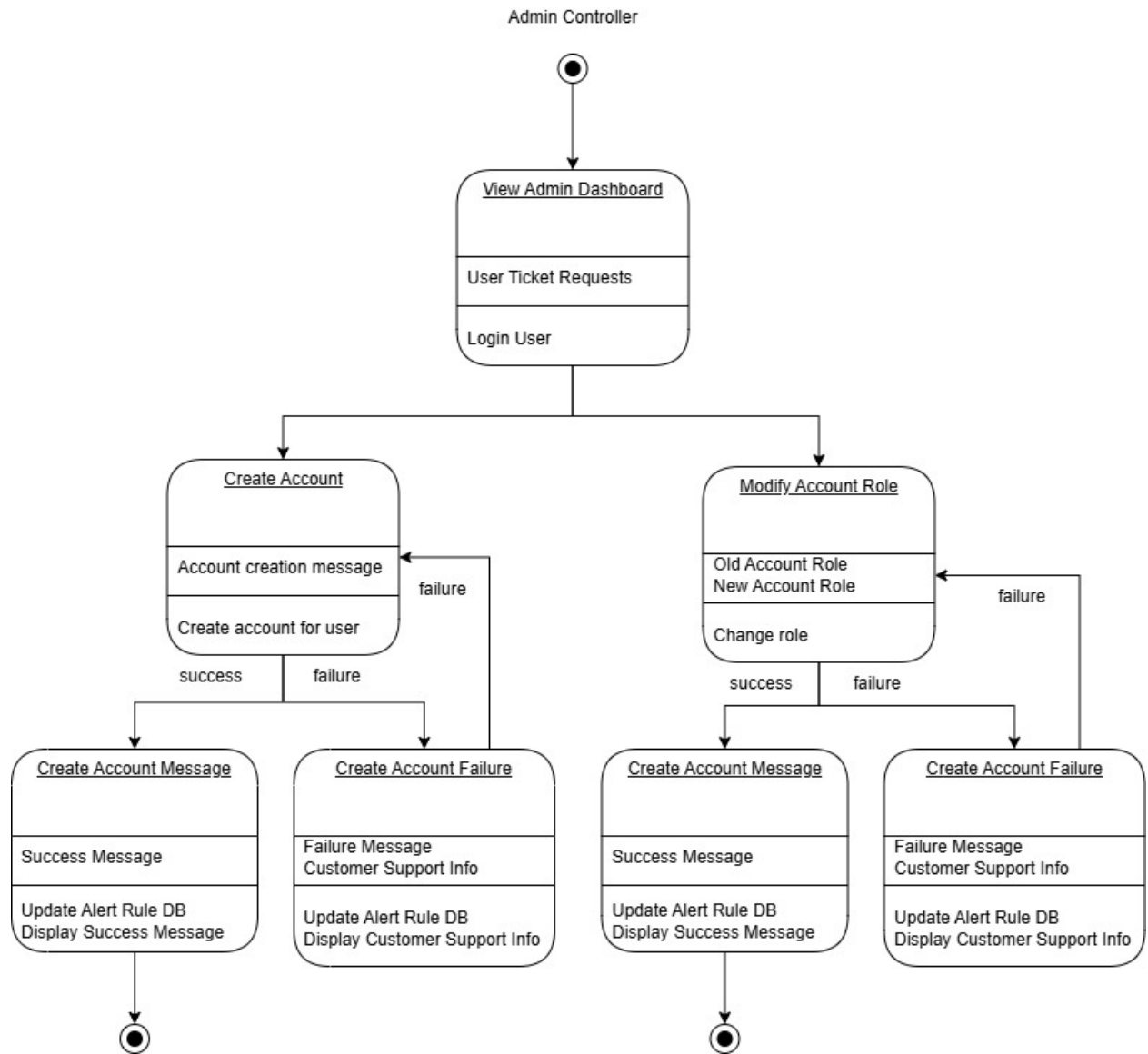
Figure 11: State diagram for Admin Controller
