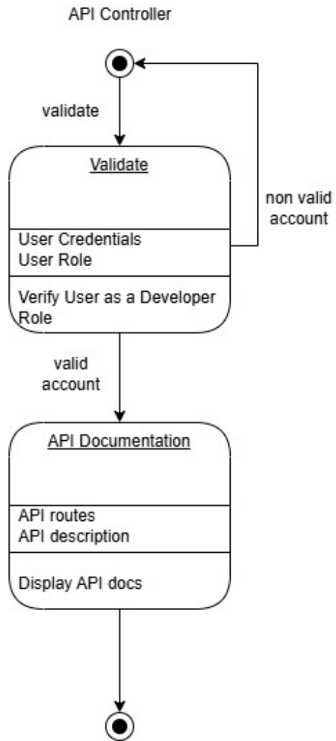
Figure 9: State diagram for API Controller
