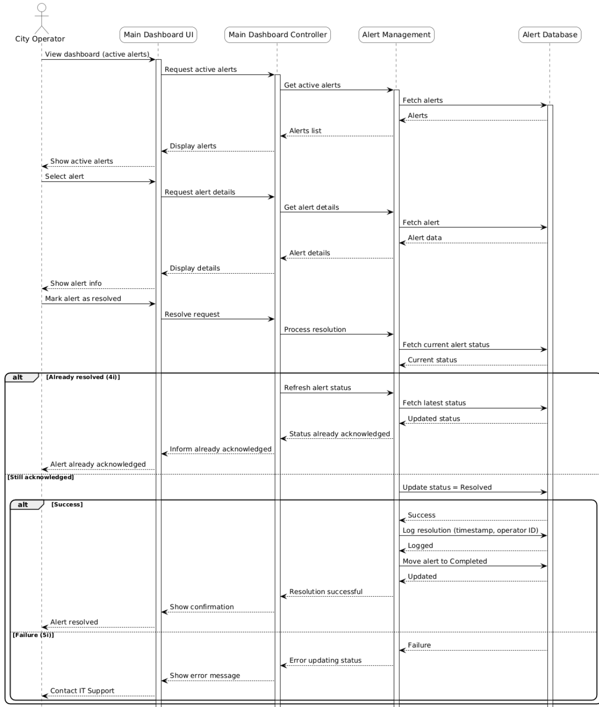
Figure 17: Sequence diagram for resolving an alert rule violation
