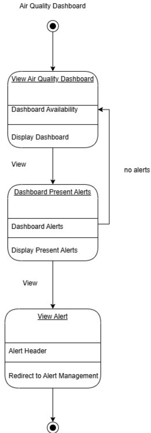
Figure 6: State diagram for Air Quality Dashboard Controller
