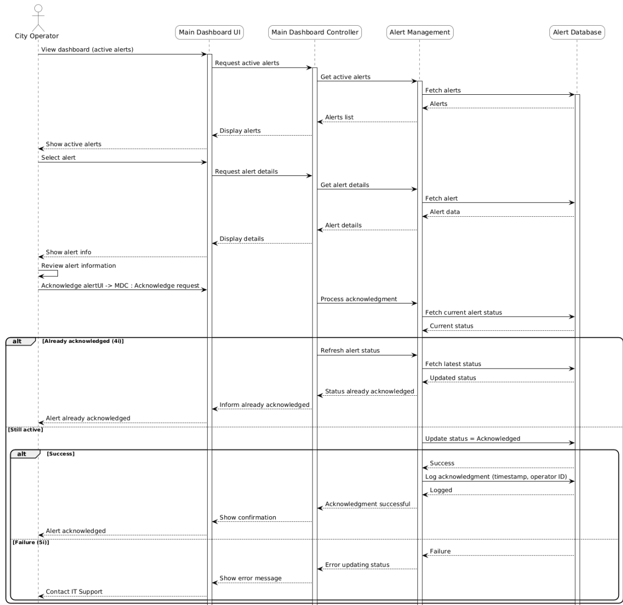
Figure 16: Sequence diagram for acknowledging a rule violation
