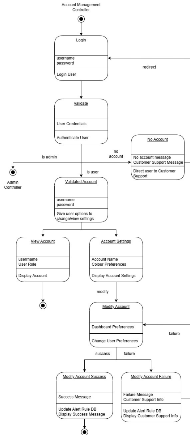
Figure 10: State diagram for Account Management Controller
