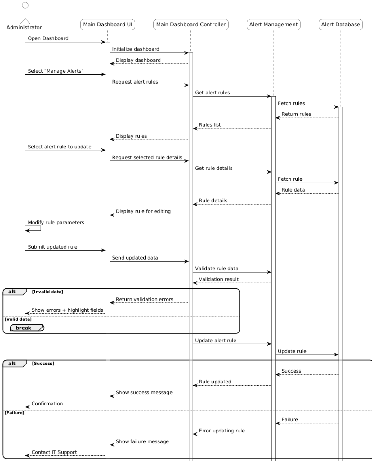
Figure 13: Sequence diagram for updating an existing alert rule
