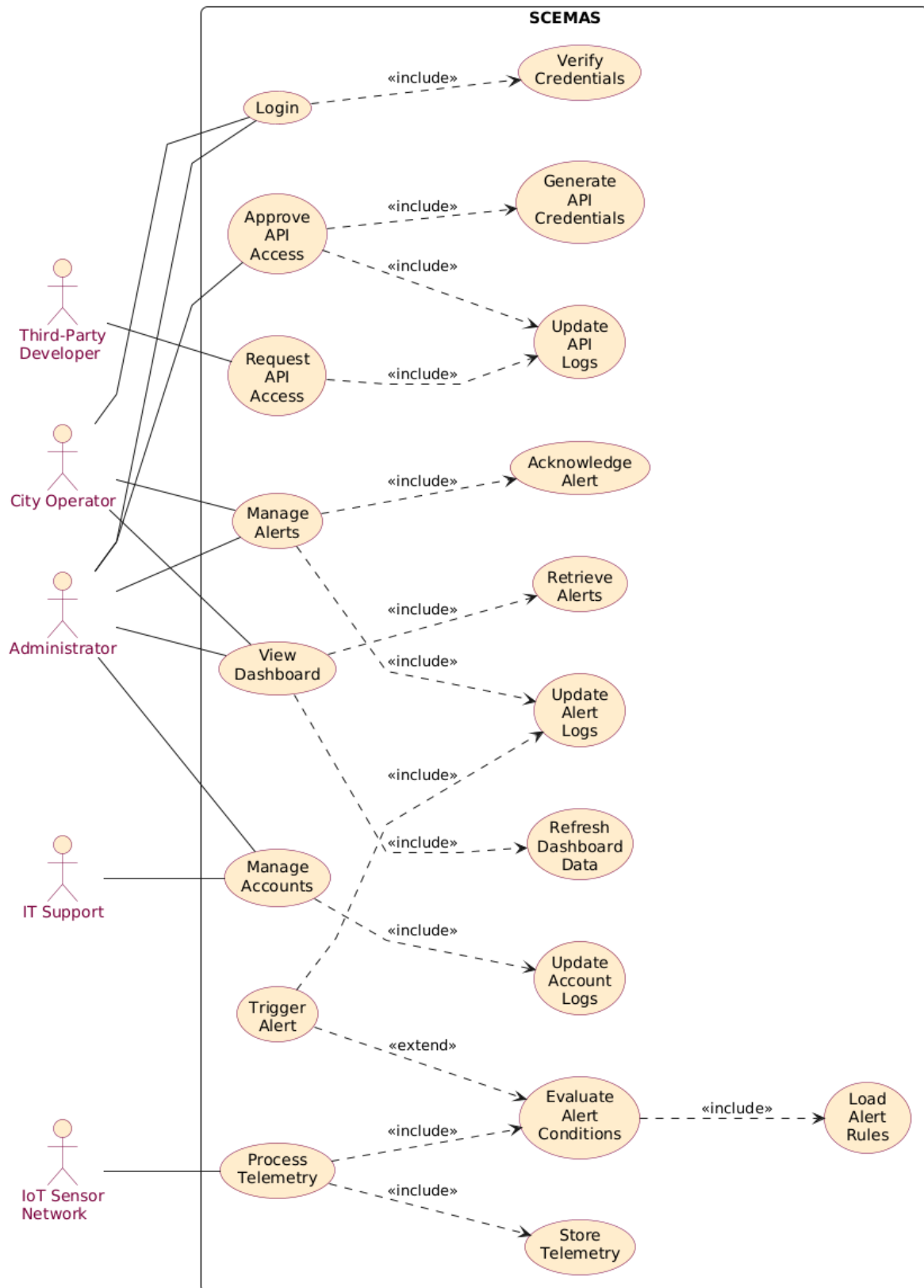
Figure 3: SCEMAS Use Case Diagram.
