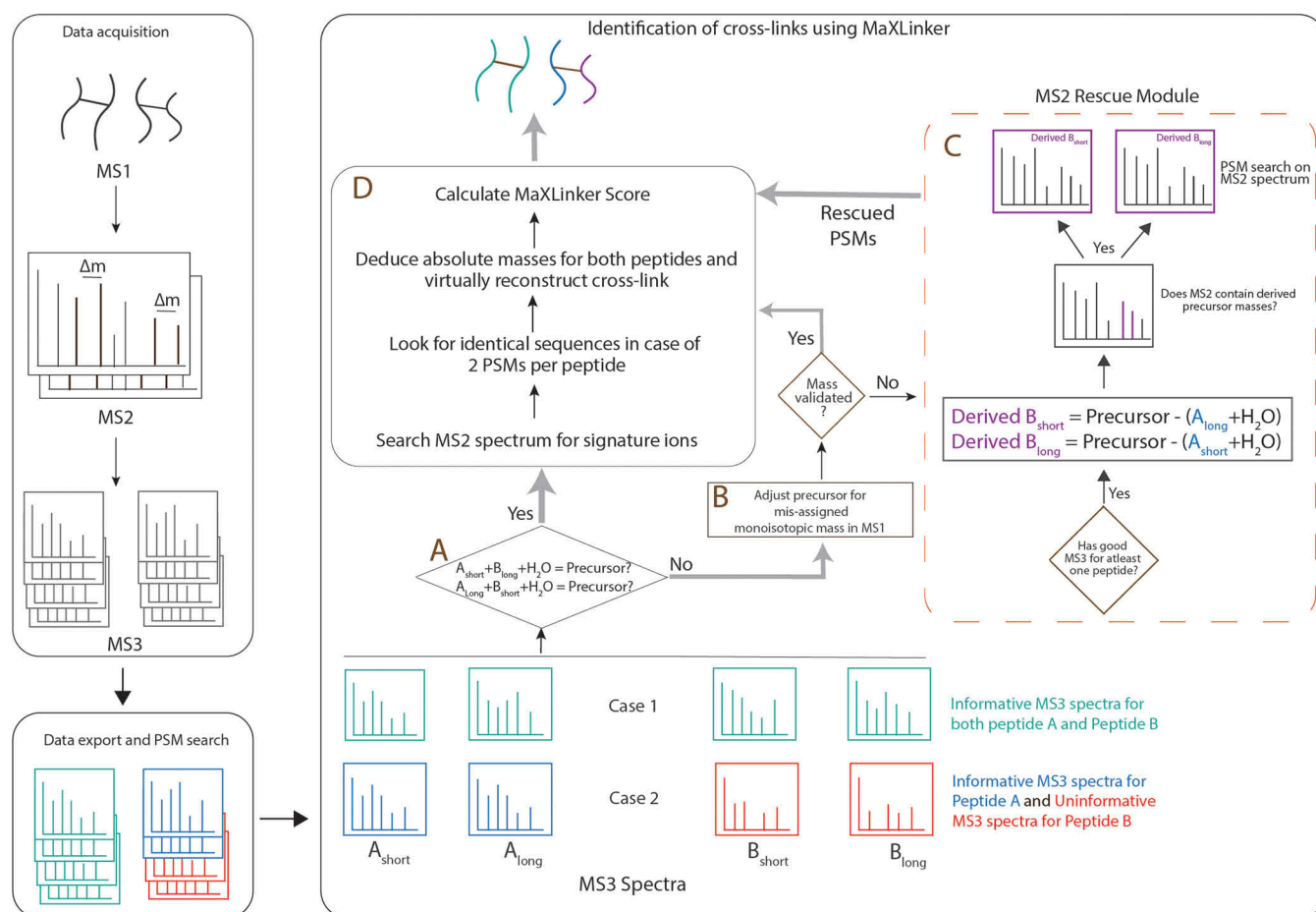
FIG. 2. Overview of MaXLinker's strategy for identification of cross-links from XL-MS.
