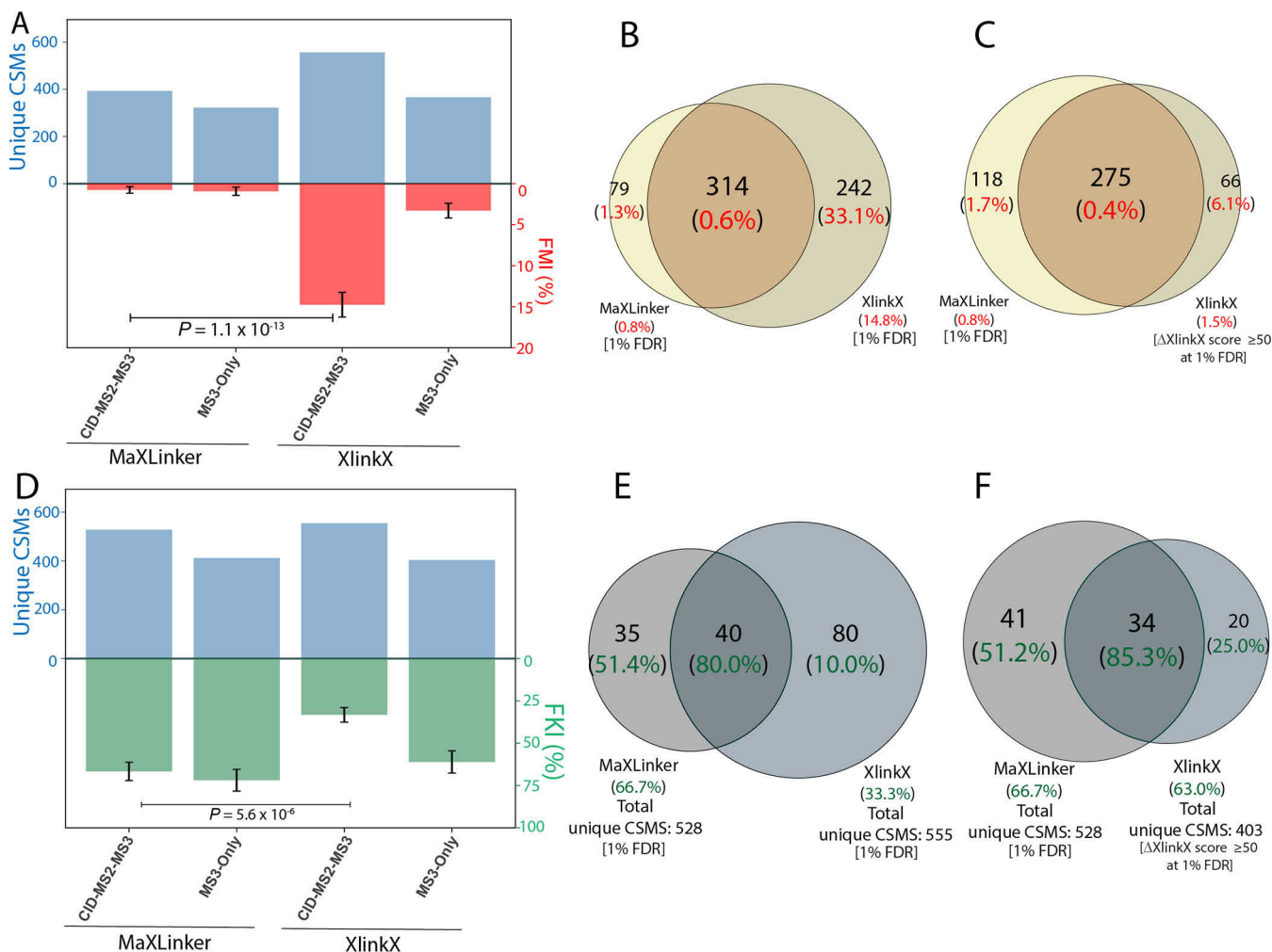
FIG. 3. Comparison of MaXLinker's performance on proteome-wide XL-MS with that of XlinkX. A, Comparison of the fraction of mis-identifications from MaXLinker and XlinkX at 1% FDR using six E. coli MS2-MS3 XL-MS fractions from Liu et al. (12). B, Overlap between CSMs from MaXLinker and XlinkX at 1% FDR showing the respective fraction of mis-identifications in the parentheses. C, Overlap between CSMs at 1% FDR from MaXLinker and additional filtering on 1% FDR with " \Delta\text{XlinkX score} \geq 50 " for XlinkX, showing the respective fraction of mis-identifications in the parentheses. D, Comparison between MaXLinker and XlinkX in terms of fraction of XLs from known interactions (FKI) using six E. coli MS2-MS3 XL-MS fractions from Liu et al. (12). E, Overlap between interprotein CSMs from MaXLinker and XlinkX at 1% FDR showing the respective FKI values in the parentheses. F, Overlap between interprotein CSMs at 1% FDR from MaXLinker and additional filtering on 1% FDR with " \Delta\text{XlinkX score} \geq 50 " for XlinkX, showing the respective FKI values in the parentheses. (Significance was determined by a two-sided Z-test; The error bars represent the estimated standard error of mean).
