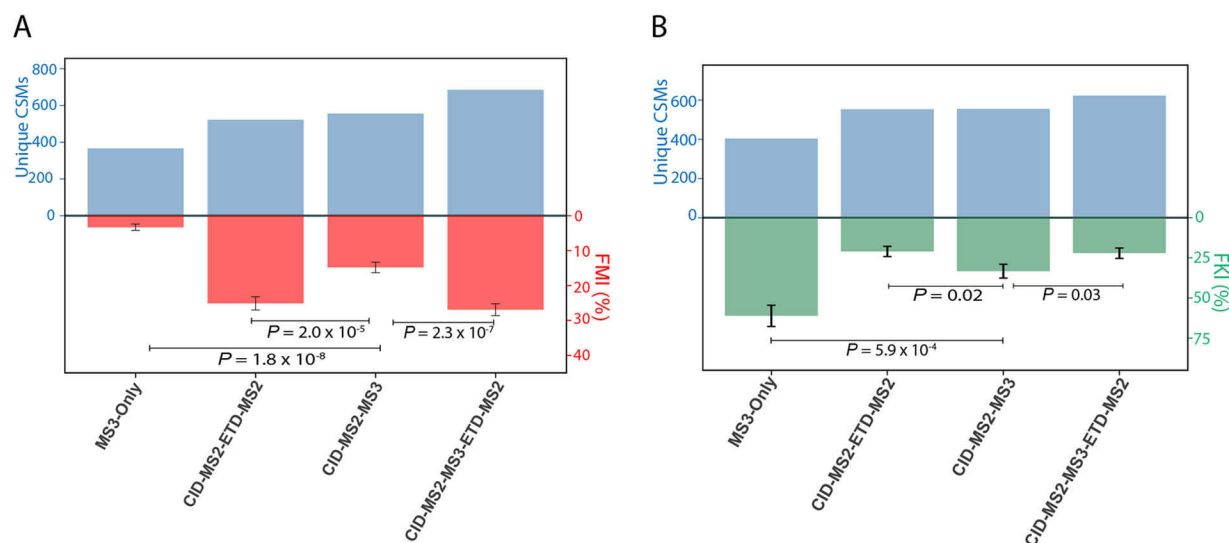
FIG. 1. Comparative quality assessment between various acquisition methods for Cross-linking Mass-Spectrometry on six E. coli fractions from Liu et al. (12) A, Comparison between different acquisition methods based on fraction of mis-identifications (FMI). (The search was performed using a database consisting amino acid sequences of E. coli and S. cerevisiae proteomes. Any CSM with either of the peptides exclusively from S. cerevisiae proteome was considered as a mis-identification). B, Quality comparison across multiple acquisition methods using the fraction of XLs from known interactions (FKI). A separate search was performed for panel “B” using only the E. coli database in order to avoid underestimation of FKI. (Significance was determined by a two-sided Z-test; The error bars represent the estimated standard error of mean).
