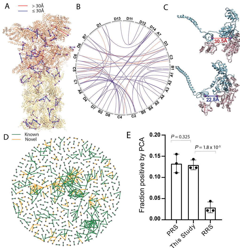
FIG. 5. Validation of cross-links and novel interactions identified in the proteome-wide human K562 XL-MS study at 1% FDR. A , Mapping cross-links from 26S proteasome complex on to a recently published structure (PDB: 5GJQ; cross-links exceeding maximum theoretical constraint 30Å are shown in red). B , A circular plot showing interprotein cross-links between various subunits from 26S proteasomal complex. (cross-links exceeding maximum theoretical constraint 30Å are shown in red; the plot was generated using Circos (57)). C , Validation of a cross-link from 26S proteasome that violate distance constraints (>30Å) in one structure (PDB: 5GJQ) and obey in a different structure (PDB: 5T0J), suggesting potential conformational changes. D , Network map showing protein-protein interactions identified in the current study. (known interactions are shown in green and novel interactions are shown in orange). E , Experimental validation of a representative set of 49 novel interactions identified in the current study using Protein-fragment complementation assay (PCA) (mean fraction positive: 0.130) (PRS: Positive Reference Set (45 interactions; mean fraction positive: 0.133); RRS: Random Reference Set (45 interactions; mean fraction positive: 0.029); The error bars represent the standard deviation; Significance was determined by a one-sided Welch Two Sample t test; 95% confidence interval; t -statistic 0.53 for “PRS - This Study,” and 164.75 for “RRS - This Study”; 2 degrees of freedom).
