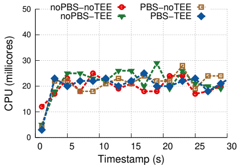
op-node
