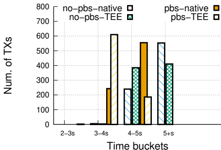
Time to inclusion
